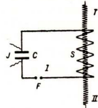
Abb. 297. Teslatriansformator
