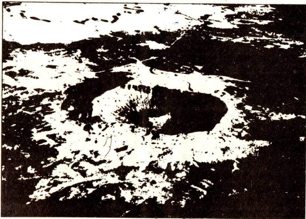
Meteoritenkrater in Arizona (USA)
