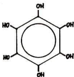
Hexahydroxybenzol
