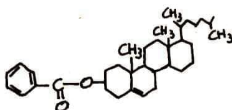
Cholesterylbenzoat
