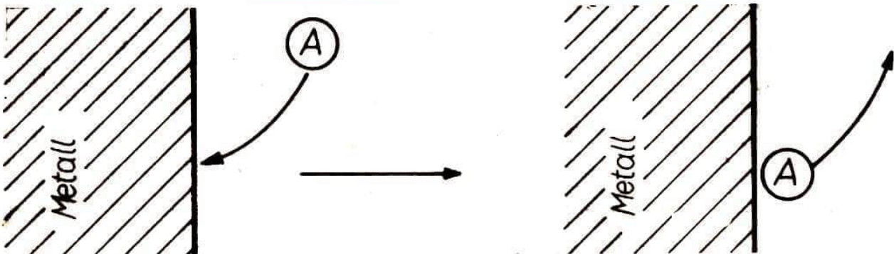
Abb. 1 Adsorption - Desorption
