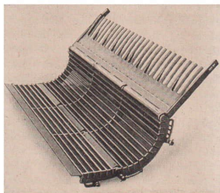
13/2 Dreschkorb
