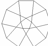
Johnson Polyeder 6
