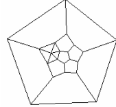
Johnson Polyeder 58
