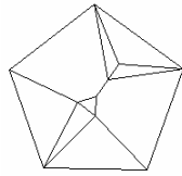
Johnson Polyeder 64
