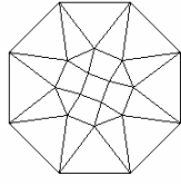
Johnson Polyeder 23
