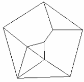
Johnson Polyeder 63
