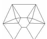
Johnson Polyeder 56
