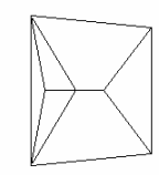
Johnson Polyeder 7
