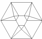
Johnson Polyeder 57
