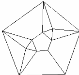
Johnson Polyeder 53
