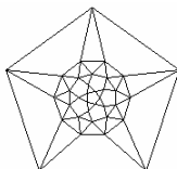
Johnson Polyeder 47
