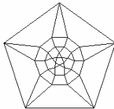
Johnson Polyeder 41
