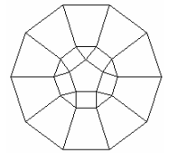
Johnson Polyeder 20
