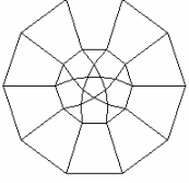
Johnson Polyeder 21
