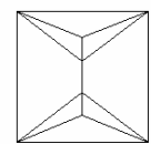
Johnson Polyeder 14
