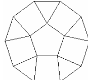
Johnson Polyeder 5
