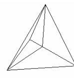
Johnson Polyeder 12
