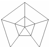
Johnson Polyeder 9
