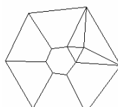
Johnson Polyeder 54
