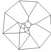
Johnson Polyeder 66
