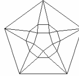
Johnson Polyeder 31
