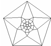
Johnson Polyeder 42
