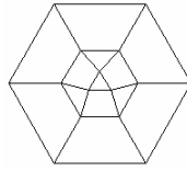
Johnson Polyeder 18
