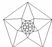
Johnson Polyeder 48
