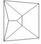
Johnson Polyeder 26
