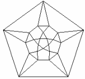
Johnson Polyeder 33
