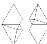
Johnson Polyeder 55
