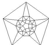
Johnson Polyeder 46
