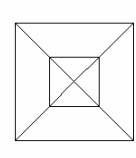
Johnson Polyeder 8
