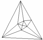
Johnson Polyeder 45
