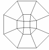
Johnson Polyeder 19
