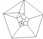
Johnson Polyeder 60
