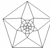
Johnson Polyeder 43
