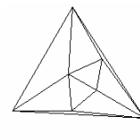
Johnson Polyeder 13
