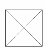
Johnson Polyeder 1
