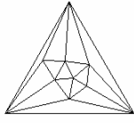
Johnson Polyeder 17
