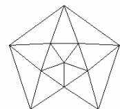
Johnson Polyeder 11
