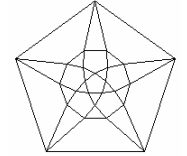
Johnson Polyeder 32
