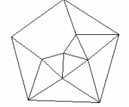
Johnson Polyeder 62
