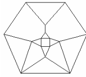
Johnson Polyeder 65
