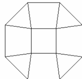
Johnson Polyeder 4
