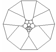
Johnson Polyeder 68
