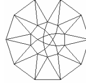
Johnson Polyeder 25
