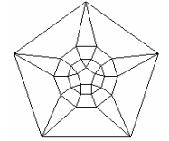
Johnson Polyeder 38
