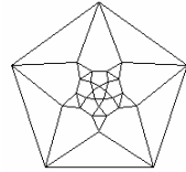
Johnson Polyeder 34
