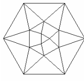
Johnson Polyeder 22
