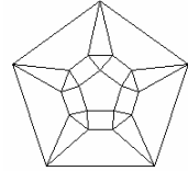
Johnson Polyeder 30
