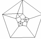
Johnson Polyeder 61
