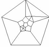
Johnson Polyeder 59
