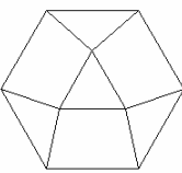
Johnson Polyeder 3
