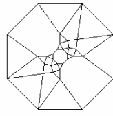
Johnson Polyeder 67
