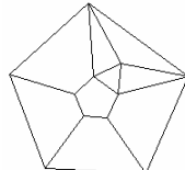
Johnson Polyeder 52
